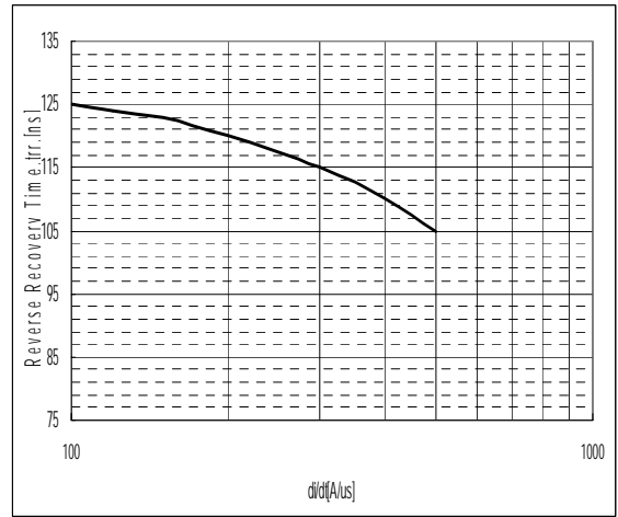
Fig. 2 : Typical Reverse Recovery Time vs. -di/dt
