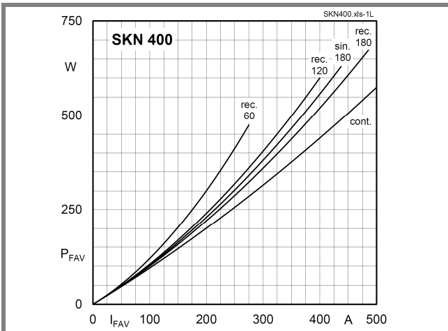
Fig. 1L Power dissipation vs. forward current
