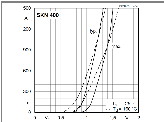
Fig. 5 Forward characteristics
