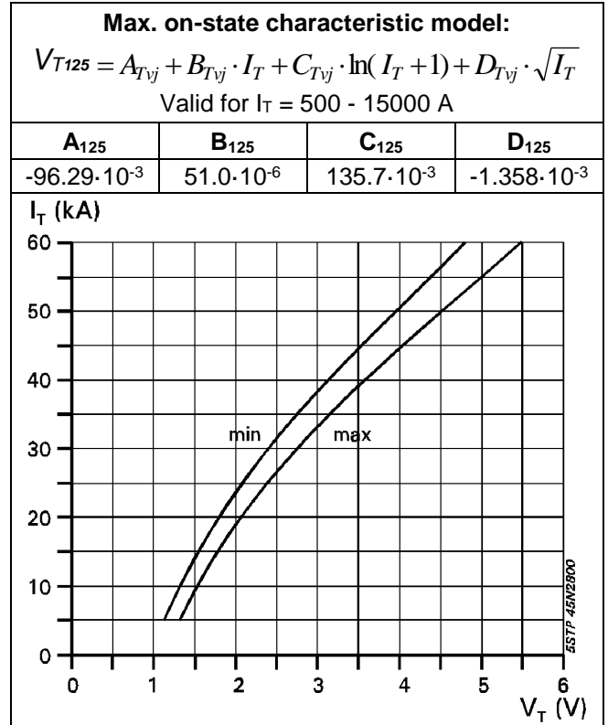
Fig. 3 On-state voltage characteristics, T_{vj} = 125 \text{ }^\circ\text{C} , 10 ms half sine
